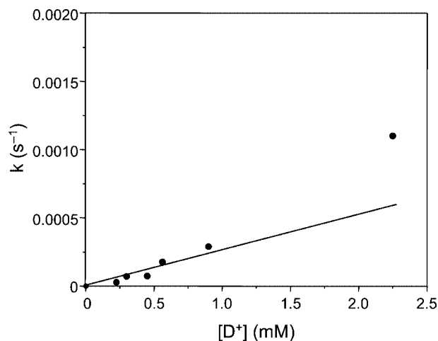
Figure 4. Relationship between DCI concentration and k_{\text{obsd.}} for derivative 2 in [\text{D}_8] -THF/water.
