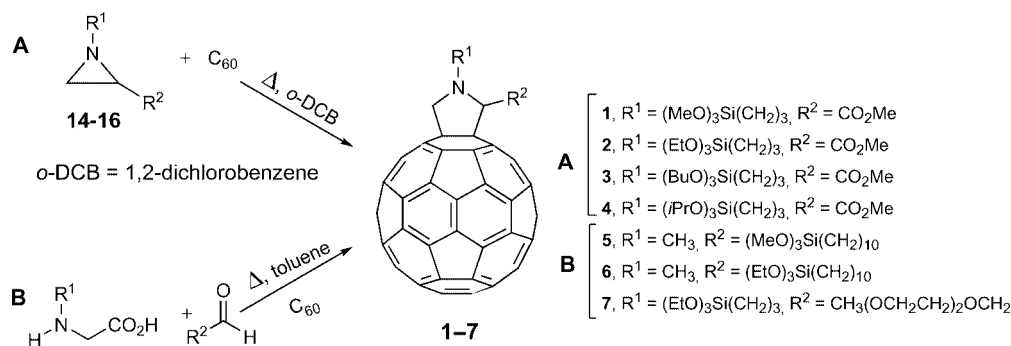
Scheme 1. Fulleropyrrolidines studied.
