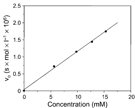
Figure 1. Initial hydrolysis rate vs. concentration for derivative 2 .
