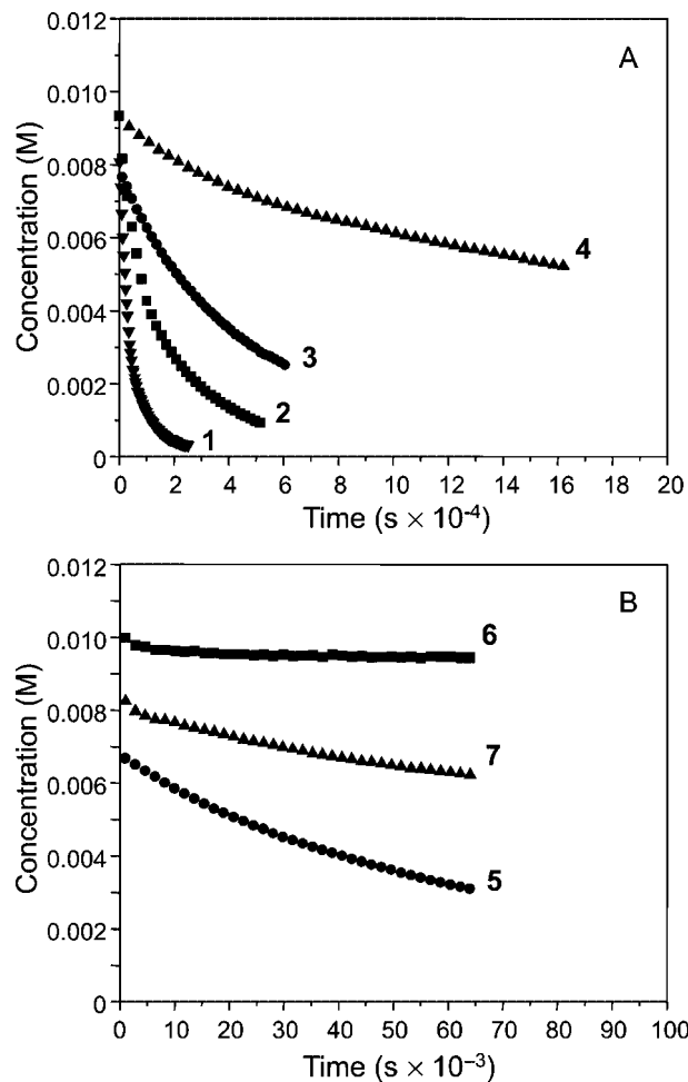
Figure 3. A) Concentration of derivatives 1–4 vs. time. B) Concentration of derivatives 5–7 vs. time.
