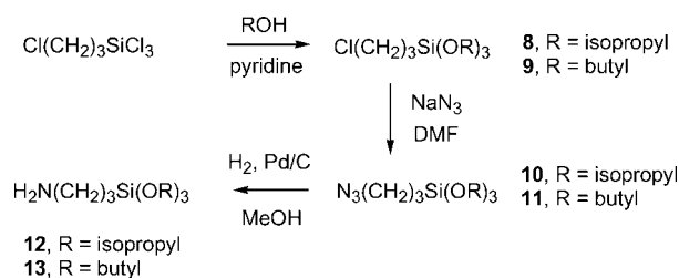
Scheme 2. Synthesis of 3-(trialkoxysilyl)propan-1-amines 12 and 13 .
