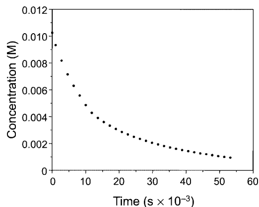
Figure 2. Plot of concentration of 2 vs. time.
